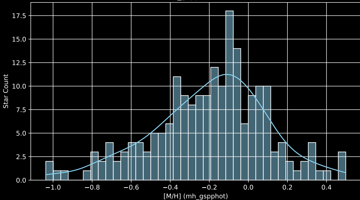
APOGEE DR17 Field: [246+49_MGA [M/H] (mh_gspphot) (n= 202)
