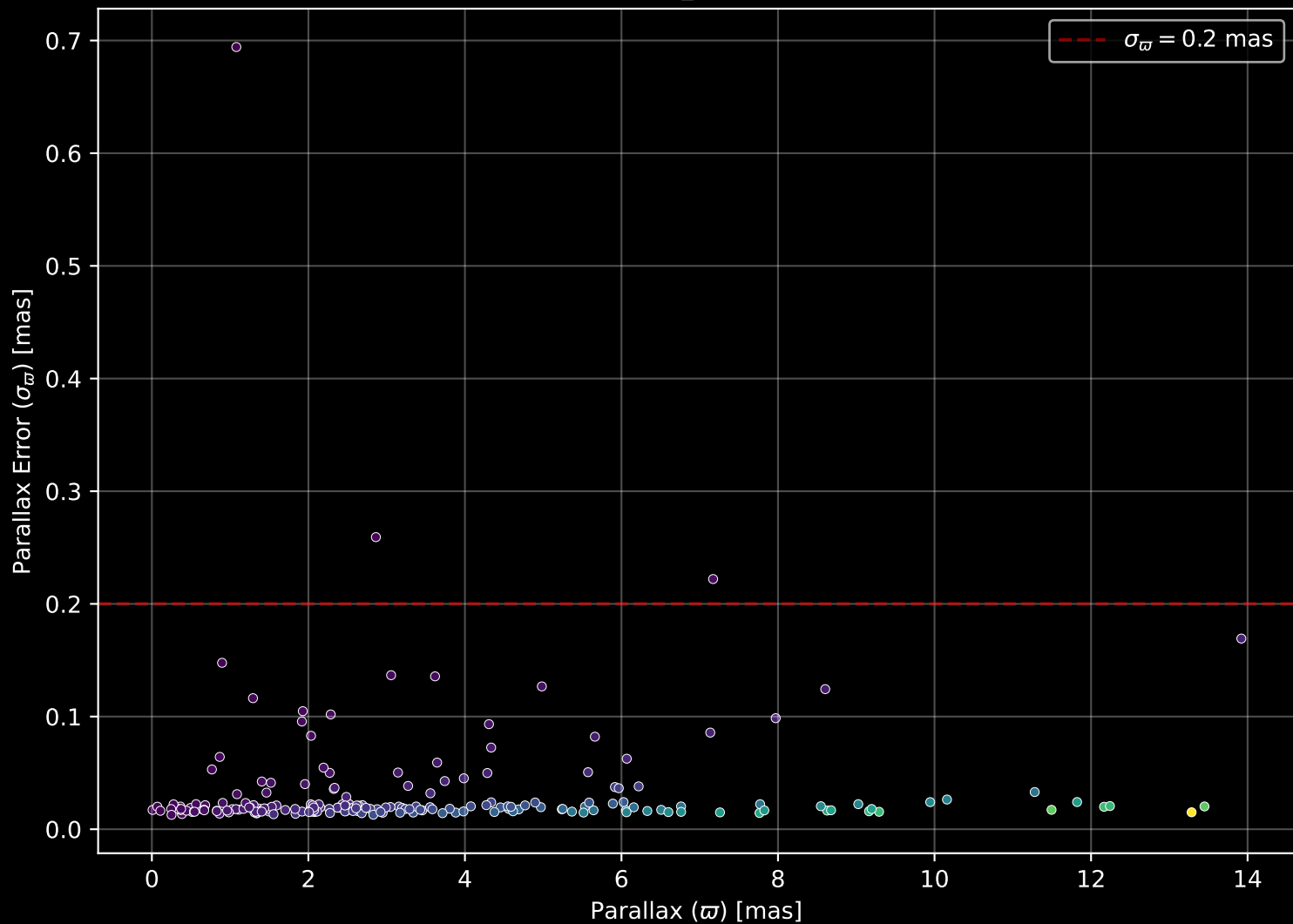
APOGEE DR17 Field: [246+49_MGA] Parallax Quality (n= 203)
