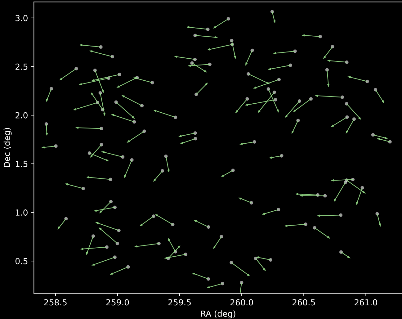
APOGEE DR17 Cluster 5 Proper Motion Vectors (n=103)
