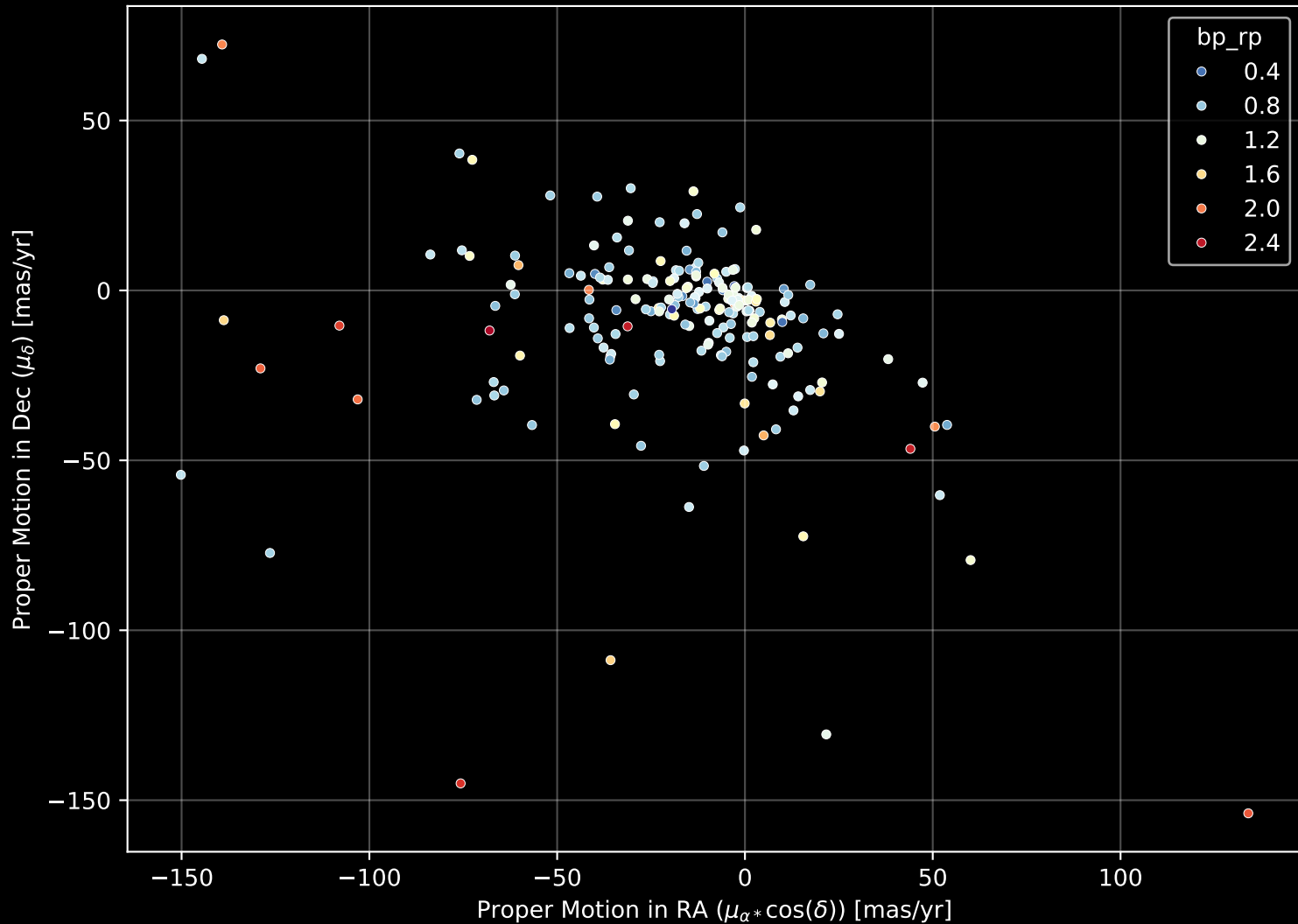
APOGEE DR17 Field: [246+49_MGA] Proper Motion Diagram (n= 203)
