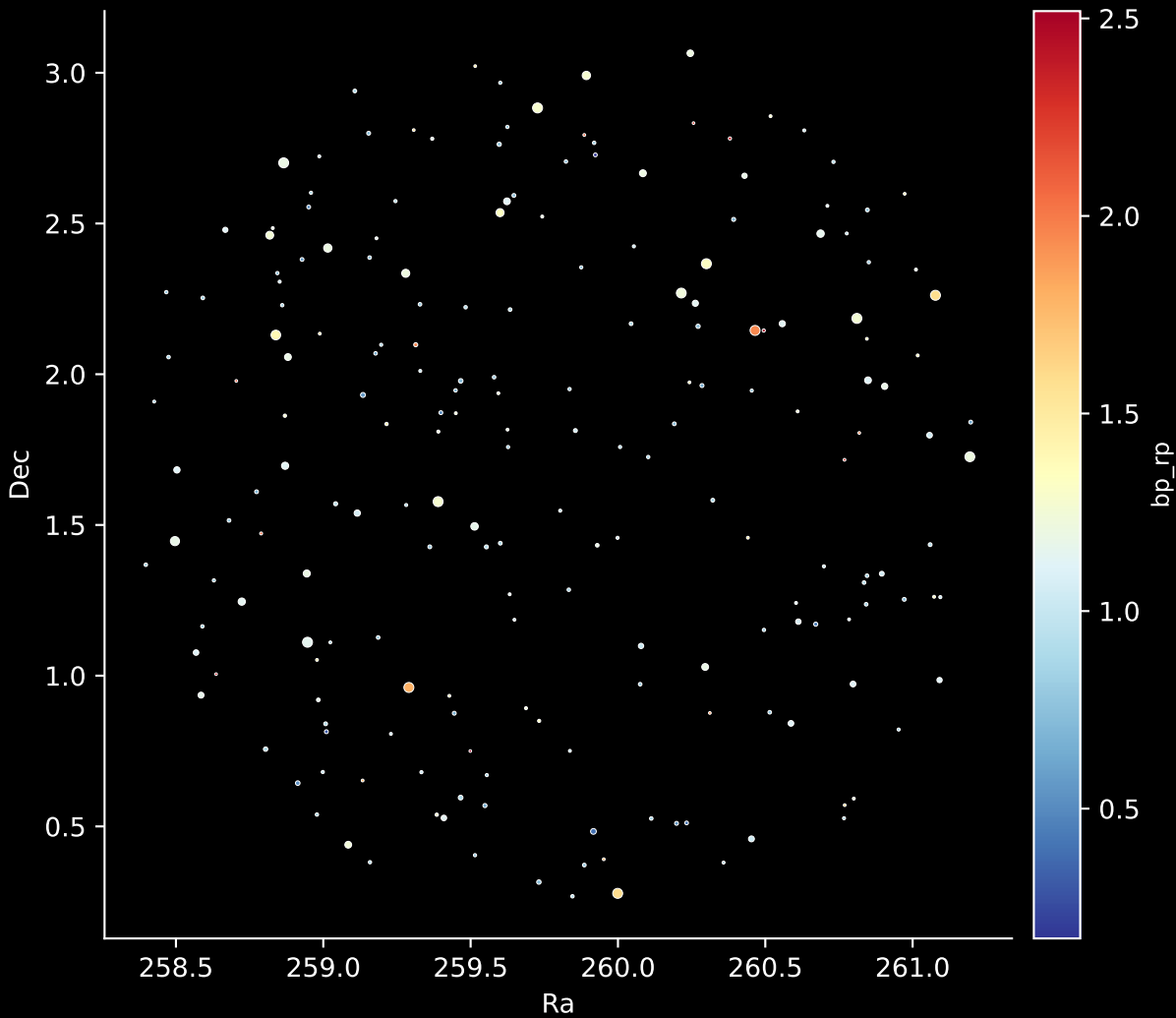
APOGEE DR17 Field: [246+49_MGA] Stars: 203
