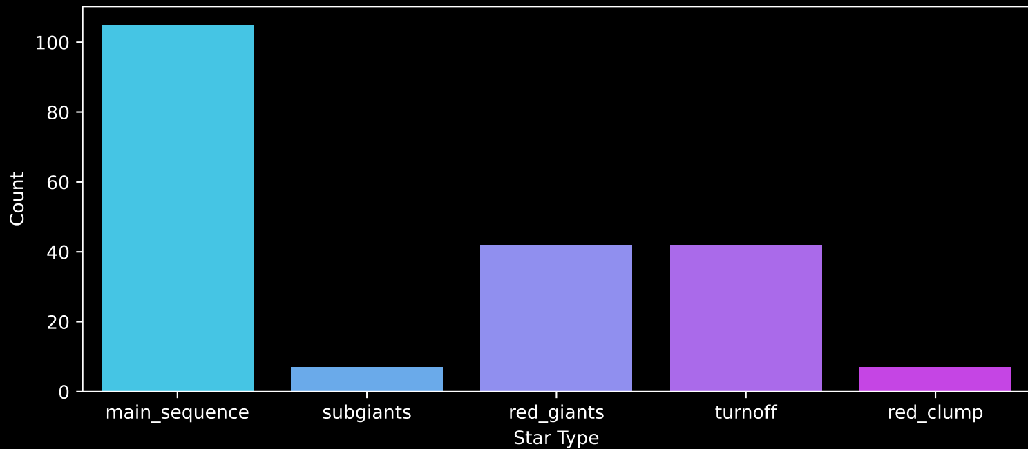
APOGEE DR17 Field: [246+49_MGA] Count plot of Star Type
