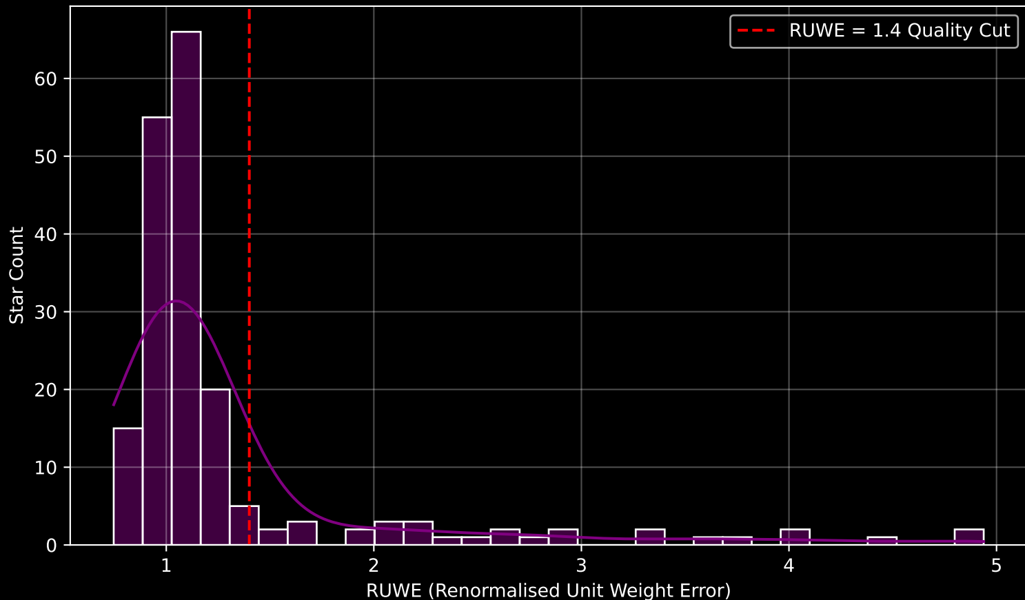
GAPOGEE DR17 Field [246+49_MGA] RUWE Distribution (n= 190)
